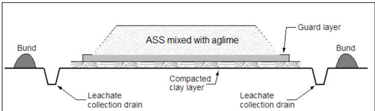
Figure 4: Schematic cross-section of a treatment pad
